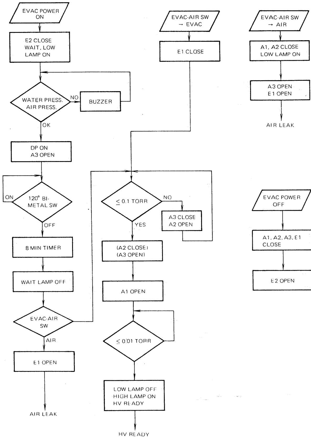
Fig. 4-2 Flowchart of Evacuation Sequence
